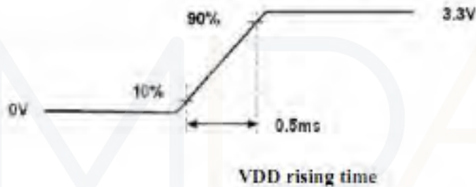
Figure 12 VDD rising time
