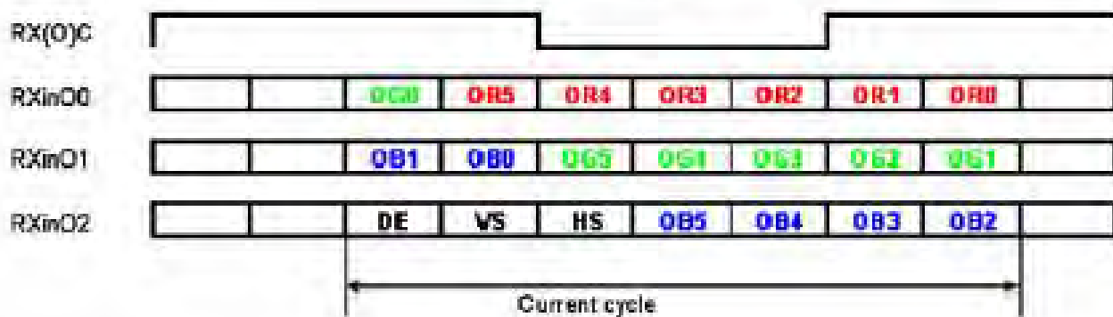
Figure 9 Data mapping
