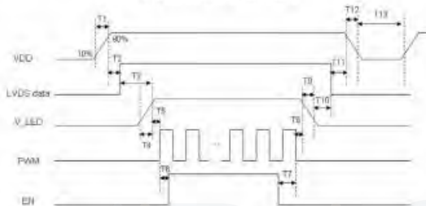
Figure 12 Power Sequence
